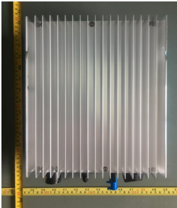
Figure 4. Back view (for EVVO 2700TL-AV, EVVO 3200TL-AV)
