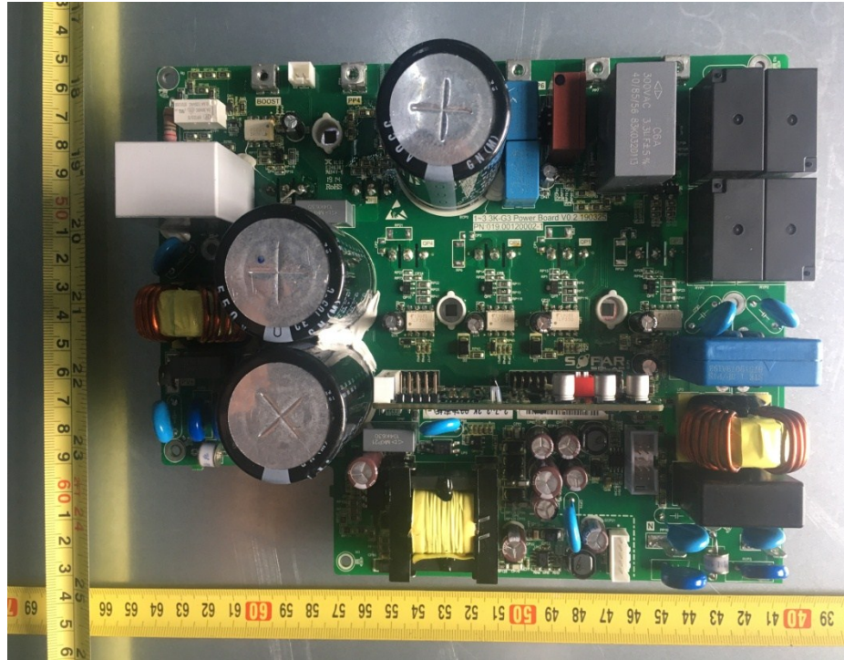
Figure 5. Front view of Main board
