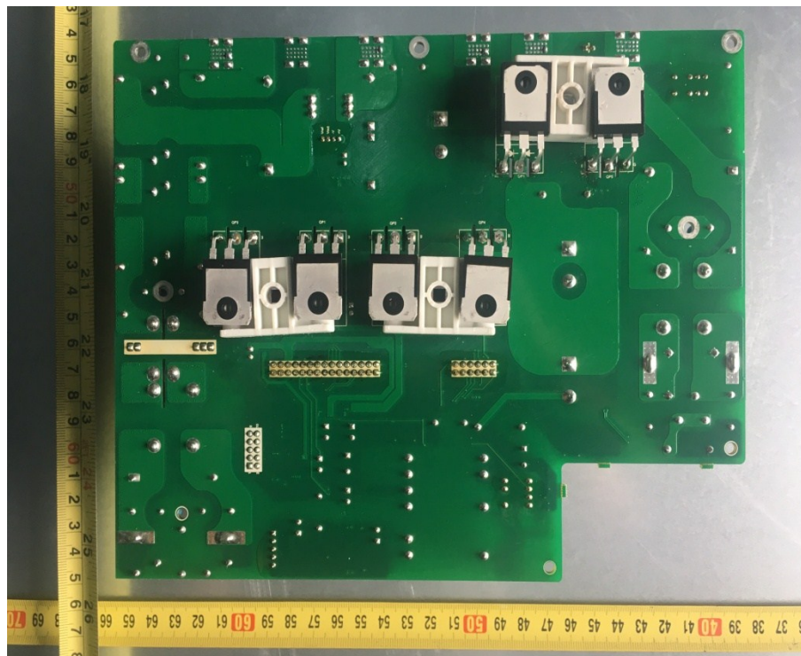
Figure 6. Back view of Main board
