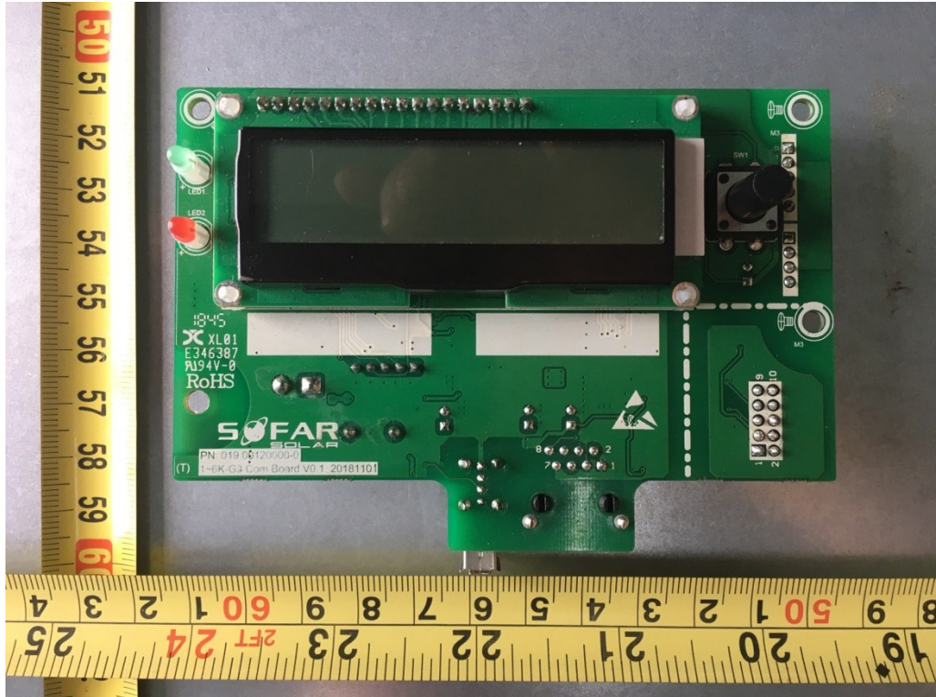
Figure 7. Front View of Display board
