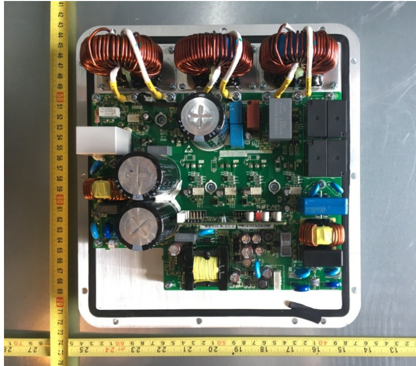
Figure 11. view of internal structure
