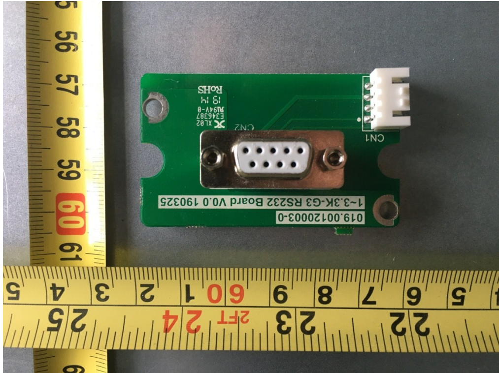
Figure 9. Front View of RS232 board
